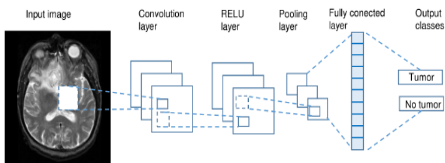
Figure 2: CNN approach.
